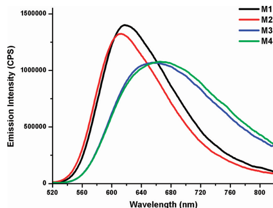
Figure 3. Photoluminescence emission spectra recorded on excitation of 10 \pm 1\text{ }\mu\text{M} acetonitrile solutions of M1–M4 at 450 nm.
