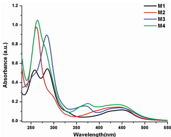
Figure 2. Absorption spectra for M1–M4 ( 10 \pm 1\text{ }\mu\text{M} ) measured in acetonitrile.
