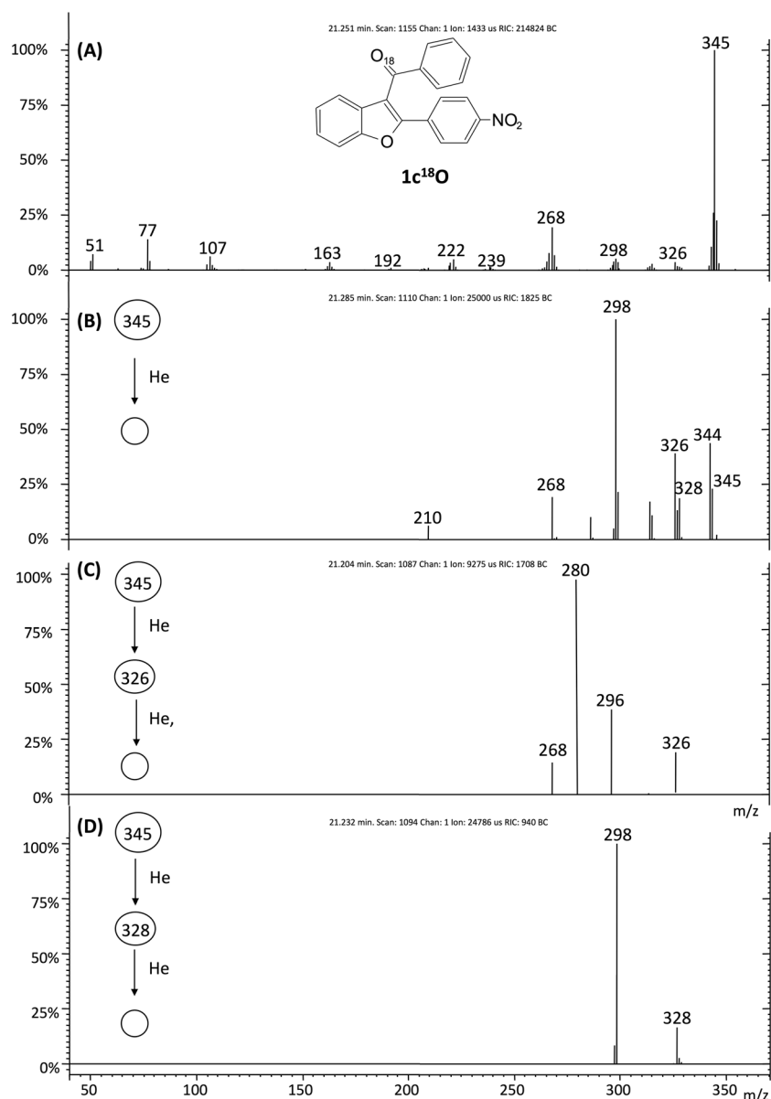
FIGURE 5 EI mass spectrum (A), MS 2 of m/z 345 (B), MS 3 of m/z 326 (C) and MS 3 of m/z 328 (D) of the labelled 3-acyl isomer 1c 18 O
