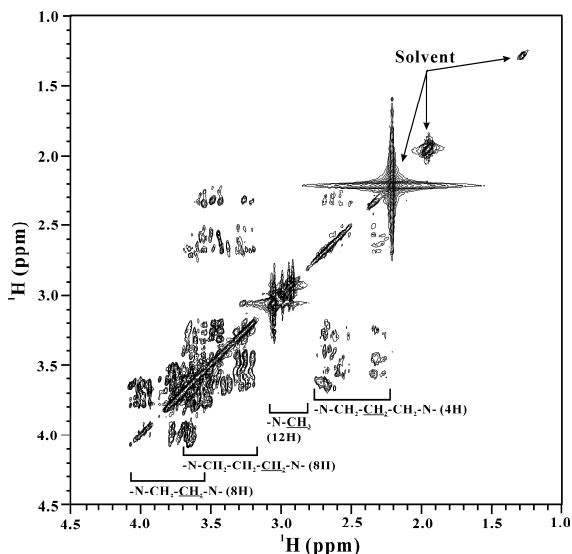
Fig. 3 2D ^1\text{H} - ^1\text{H} -COSY spectrum of 1 in \text{CD}_3\text{CN} at 25^\circ\text{C} .
