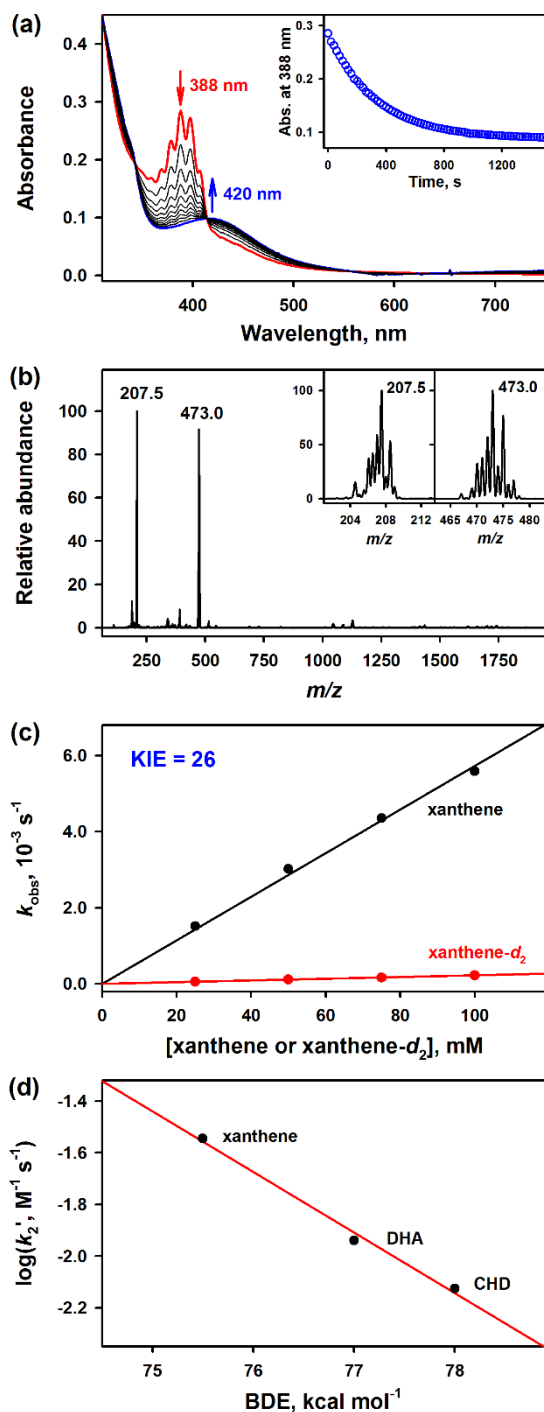
Fig. 5 (a) UV-vis spectral changes of 1 (0.50 mM) upon addition of xanthene (50 mM) at 35 °C. Inset shows time course of the decay of 1 monitored at 388 nm. (b) ESI-MS spectrum of the reaction solution obtained in the reaction of 1 (1.0 mM) with xanthene (50 mM) in CH 3 CN at 35 °C. The peaks at m/z = 207.5 and 473.0 correspond to [Ru IV (TMC)(O)(CH 3 CN)] 2+ (calc. m/z = 207.6 ) and [Ru IV (TMC)(O)(ClO 4 )] + (calc. m/z = 473.1 ), respectively. Insets show the isotopic distribution patterns of the peaks at m/z = 207.5 and 473.0. (c) Plots of k_{\text{obs}} against concentrations of xanthene and xanthene- d 2 to determine the KIE value of 26(2). (d) Plot of \log k_2' of 1 against C-H BDE of substrates. Second-order rate constants ( k_{\text{HAT}} ) were determined at 35 °C and then adjusted for reaction stoichiometry to yield k_2' based on the number of equivalent target C-H bonds of substrates (e.g., 2 for xanthene and 4 for DHA and CHD).
