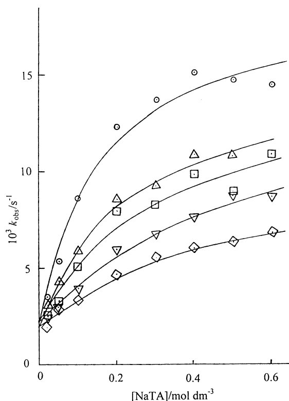
Fig. 1 Plots showing the dependence of k_{\text{obs}} upon [\text{NaTA}] where NaTA represents sodium o -toluate at 0.005 ( \circ ), 0.007 ( \Delta ), 0.010 ( \square ), 0.015 ( \nabla ) and 0.020 \text{mol dm}^{-3} ( \diamond ) CTABr. The solid lines are drawn through the least-squares calculated points.
