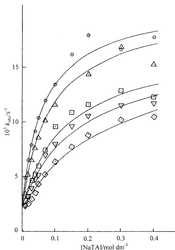
Fig. 2 Plots showing the dependence of k_{\text{obs}} upon [\text{NaTA}] where NaTA represents sodium m -toluate at 0.005 ( \circ ), 0.007 ( \Delta ), 0.010 ( \square ), 0.015 ( \nabla ) and 0.020 \text{mol dm}^{-3} ( \diamond ) CTABr. The solid lines are drawn through the least-squares calculated points.
