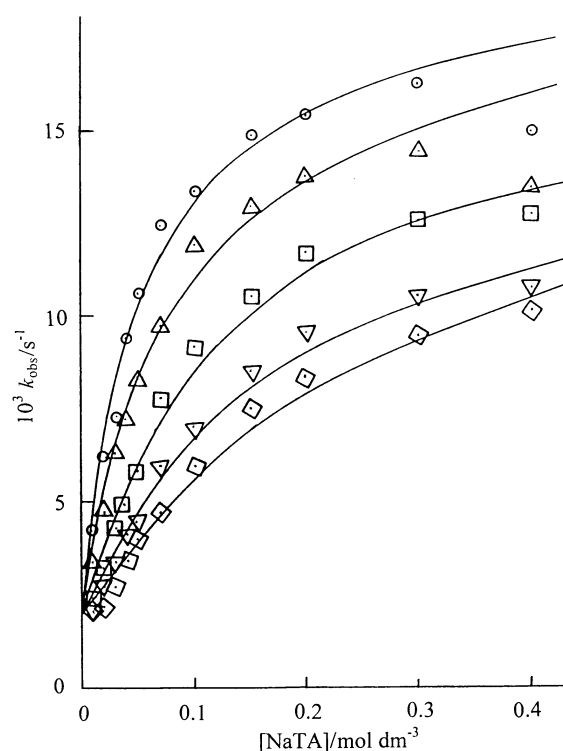
Fig. 3 Plots showing the dependence of k_{\text{obs}} upon [\text{NaTA}] where NaTA represents sodium p -toluate at 0.005 ( \circ ), 0.007 ( \Delta ), 0.010 ( \square ), 0.015 ( \nabla ) and 0.020 \text{mol dm}^{-3} ( \diamond ) CTABr. The solid lines are drawn through the least-squares calculated points.
