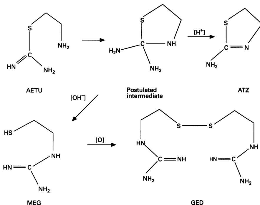
Figure 11 Scheme demonstrating the rearrangement of aminoethyl-isothioureia (AETU) to aminothiazoline (ATZ) and mercaptoethylguanidine (MEG) and the subsequent dimerization of MEG to guanidinoethyldisulphide (GED).
