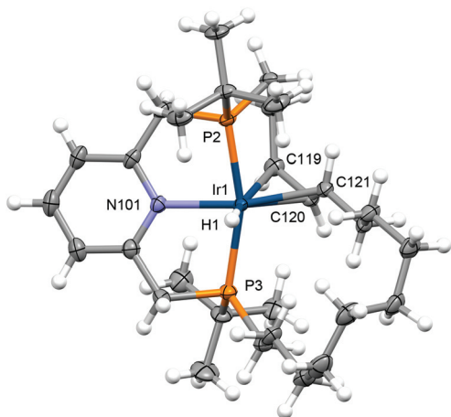
Fig. 1 Solid-state structure of 7 : the hydride ligand was located from the Fourier difference map; thermal ellipsoids at 30% probability; solvent molecule and anion omitted. Selected bond lengths (Å) and angles (°): Ir1–P2, 2.2694(8); Ir1–P3, 2.3339(9); P2–Ir1–P3, 163.04(3); Ir1–N101, 2.126(2); Ir1–H1, 1.39(3); Ir1–C119, 2.311(4); Ir1–C120, 2.155(3); Ir1–C121, 2.199(3); C119–C120, 1.430(5); C120–C121, 1.409(5); C119–C120–C121, 124.4(3); N101–Ir1–C121, 169.59(11).
