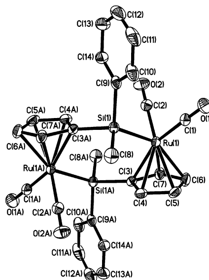
Figure 1. ORTEP diagram of 7 . Thermal ellipsoids are shown at the 30% level.
