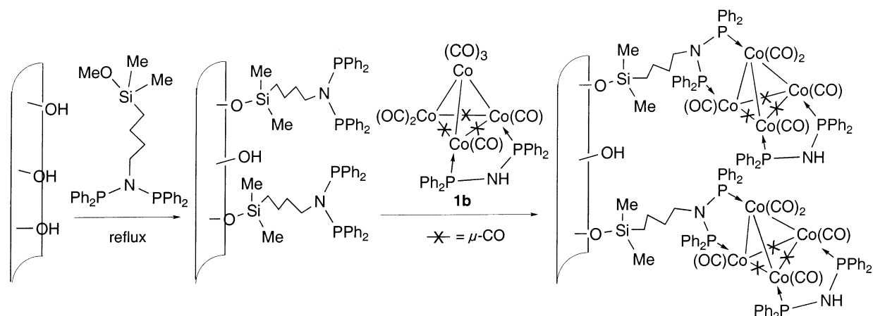
Scheme 1. Anchoring of a Co 4 Cluster into Functionalized Alumina Membranes 7
