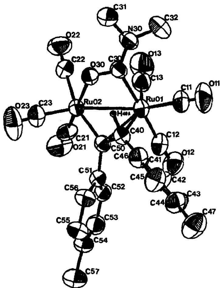
Fig. 6. ORTEP projection of \text{Ru}_2\{\mu\text{-O}=\text{C}(\text{NMe}_2), \mu\text{-}\sigma, \pi\text{-C}(p\text{-tolyl})=\text{CH}(p\text{-tolyl})\}(\text{CO})_6 , 3b ; thermal ellipsoids at 50% probability.
