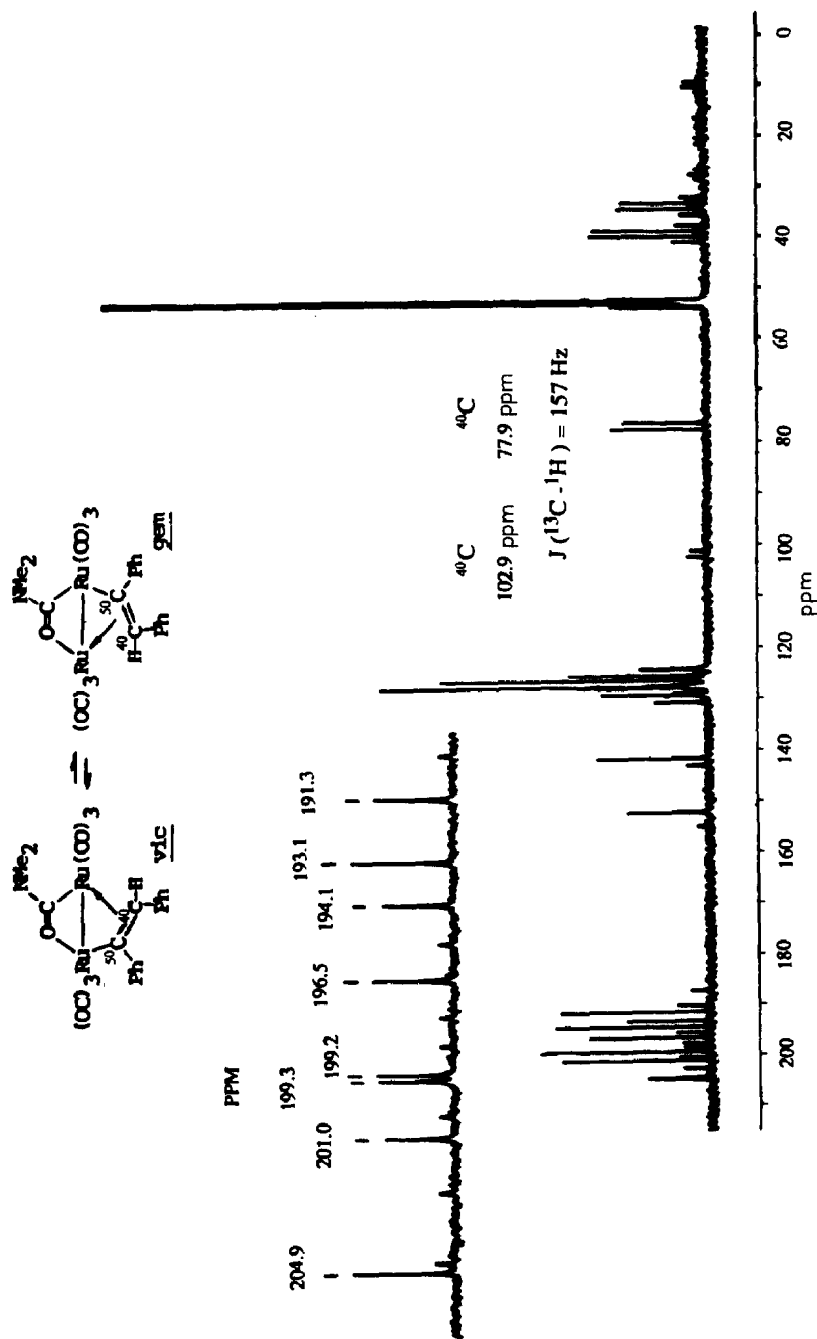
Fig. 2. ^{13}\text{C} NMR at 125.8 MHz of \text{Ru}_2\{\mu\text{-O-C}(\text{NMe}_2)\}_2\mu\text{-}\sigma\text{-C}(\text{Ph})=\text{C}(\text{H})\text{Ph}\}(\text{CO})_6 , 3a , -50^\circ\text{C} , \text{CD}_2\text{Cl}_2 solution. Insert. Peak positions of the resonances of the minor isomer are, respectively: 204.6, 202.6, 200.4, 198.4, 197.6, 195.7, 190.2, 187.1.
