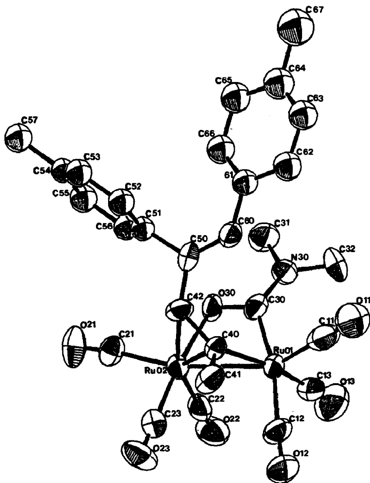
Fig. 7. ORTEP projection of \text{Ru}_2\{\mu\text{-O}=\text{CNMe}_2, \mu\text{-}\sigma, \pi\text{-C}(\text{CH}_3)=\text{C}(\text{H})\text{C}(\textit{p}\text{-tolyl})=\text{CH}(\textit{p}\text{-tolyl})\}(\text{CO})_6 , 5 ; thermal ellipsoids at 50% probability.
