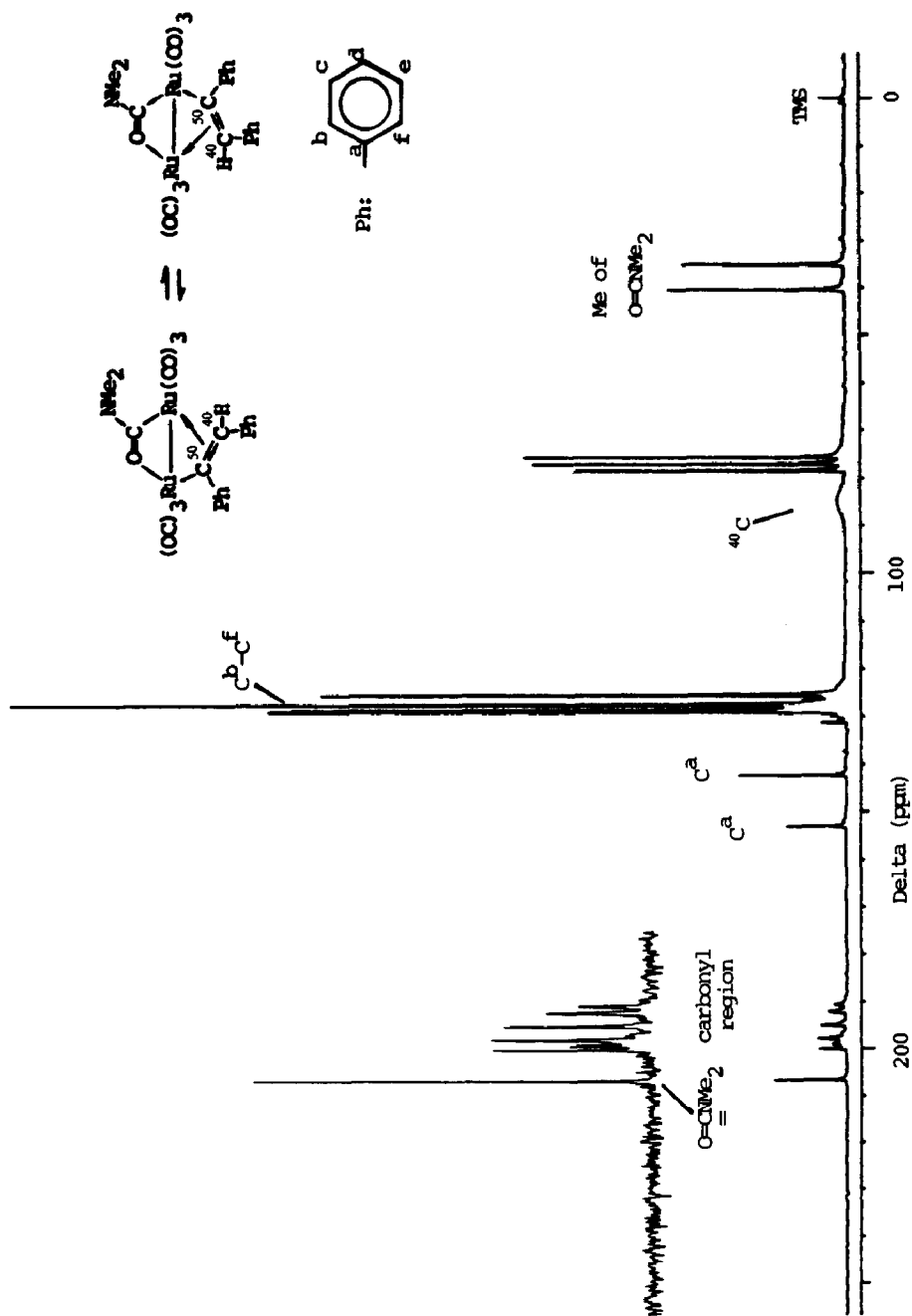
Fig. 4. ^{13}\text{C}\{^1\text{H}\} NMR at 22.5 MHz of \text{Ru}_3\{\mu\text{-O}=\text{C}(\text{NMe}_2)\}_2\mu\text{-}\sigma\text{-}\pi\text{-C}(\text{Ph})=\text{C}(\text{H})(\text{Ph})\}(\text{CO})_6 , 3a , +30^\circ\text{C} , \text{CDCl}_3 solution.
