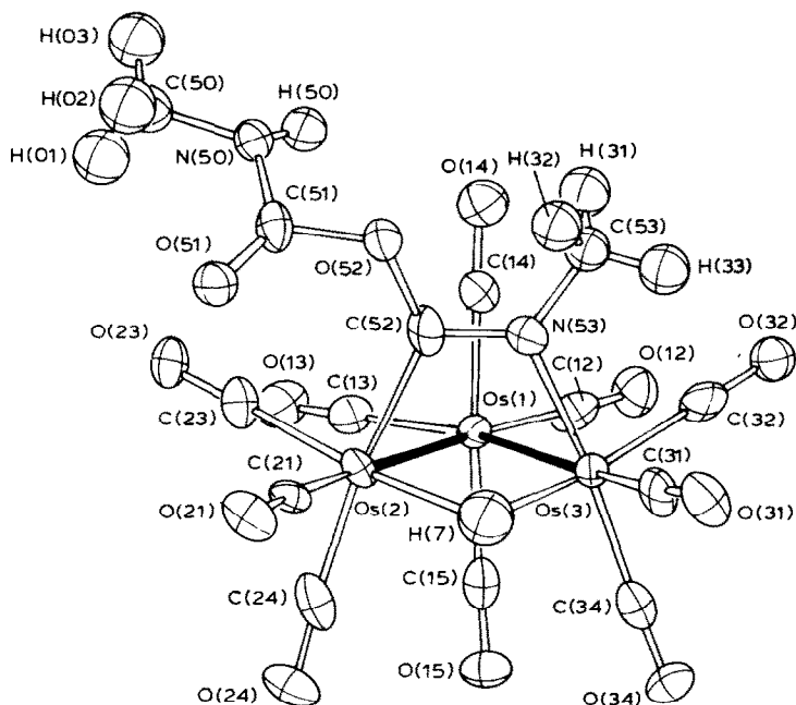
Fig. 2. ORTEP projection of \text{HOs}_3(\mu\text{-C(OR)=NMe})(\text{CO})_{10} , \text{R} = \text{C(O)N(H)Me} ; thermal ellipsoid at 50% probability.
