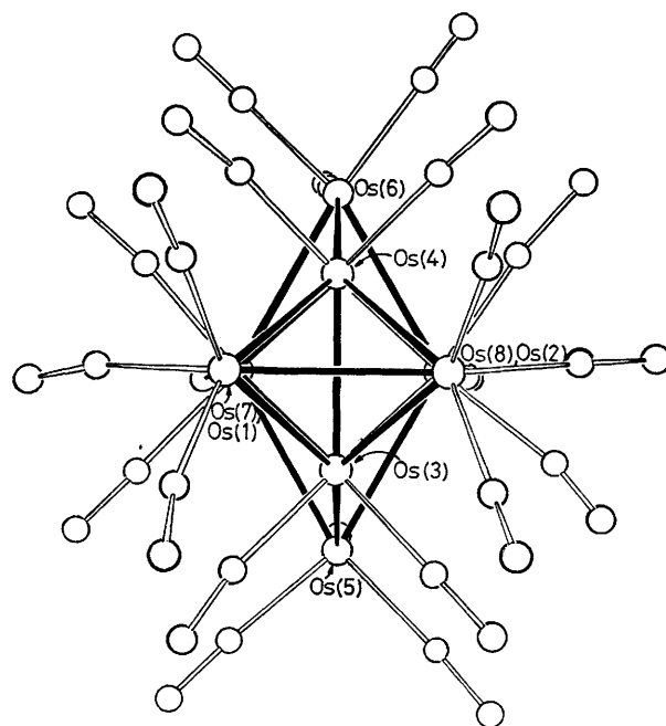
Figure 2. The anion [\text{HOs}_8(\text{CO})_{22}]^- viewed down the virtual C_2 axis. The H-ligand bridges Os(7)-Os(8).
