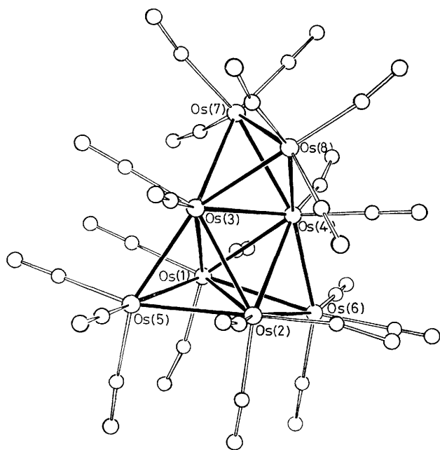
Figure 1. The structure of the anion [\text{HOs}_8(\text{CO})_{22}]^- (1). Os-Os bond lengths (those for the [\text{Ph}_3\text{PMe}]^+ salt are given first and those for the [\text{PPN}]^+ salt are in parentheses): (1)-(2) 2.740, (2.758); (1)-(3) 2.842, (2.823); (1)-(4) 2.829, (2.825); (1)-(5) 2.866, (2.842); (1)-(6) 2.854, (2.850); (2)-(3) 2.837, (2.842); (2)-(4) 2.839, (2.840); (2)-(5) 2.861, (2.845); (2)-(6) 2.868, (2.872); (3)-(4) 2.600, (2.606); (3)-(5) 2.723, (2.702); (3)-(7) 2.783, (2.801); (3)-(8) 2.805, (2.805); (4)-(6) 2.710, (2.711); (4)-(7) 2.803, (2.735); (4)-(8) 2.734, (2.800); (7)-(8) 2.848, (2.842). Maximum e.s.d.'s are 0.001 Å for the [\text{Ph}_3\text{PMe}]^+ salt and 0.004 Å for the [\text{PPN}]^+ salt.
