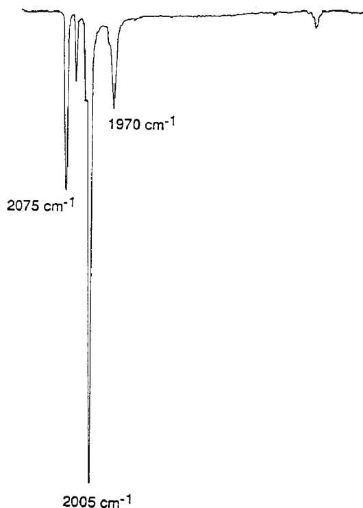
Fig. 2. Infrared spectrum in the carbonyl region for the hexane extract from the room-temperature reaction of [\text{Ni}_6(\text{CO})_{12}]^{2-} dianion (1) with \text{Ph}_2\text{SbCl} . Relatively strong bands at 2075 and 2005\text{ cm}^{-1} are assigned to \text{Ni}(\text{CO})_3(\text{SbClPh}_2) , the weaker bands at 2020 and 1970\text{ cm}^{-1} to \text{Ni}_2(\text{CO})_4(\mu_2\text{-Ph}_2\text{SbOSbPh}_2) (3), and the band at 2040\text{ cm}^{-1} to \text{Ni}(\text{CO})_4 . These assignments are based upon comparative infrared spectra either of these species per se and/or of closely related species.
