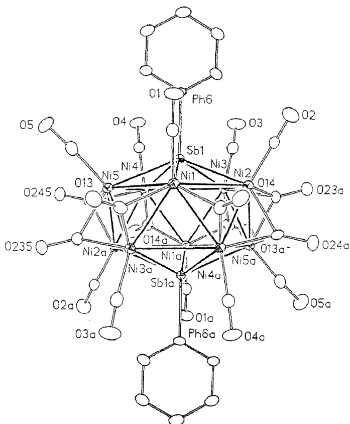
Fig. 5. Configuration of the [\text{Ni}_{10}(\text{SbPh})_2(\text{CO})_{18}]^{2-} dianion of the acetone-solvated [\text{NMe}_4]^+ salt ( 2b ). The entire dianion of crystallographic C_i-1 site symmetry closely conforms to C_{2h}-2/m symmetry with the pseudo mirror plane passing through \text{Ni}(1) , \text{Ni}(1a) , \text{Sb}(1) , \text{Sb}(1a) and symmetry relating the \text{Ni}(2) , \text{Ni}(5) atoms and the \text{Ni}(3) , \text{Ni}(4) atoms. The anisotropic thermal ellipsoids are drawn at the 35% probability level.
