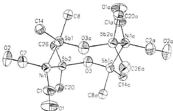
Fig. 7. Configuration of the \text{Ni}_2(\text{CO})_4(\mu_2\text{-Ph}_2\text{SbOSbPh}_2)_2 molecule ( 3 ) possesses crystallographic C_i -1 site symmetry. Only the Sb-attached carbon atom for each of the eight phenyl substituents is shown (for clarity).
