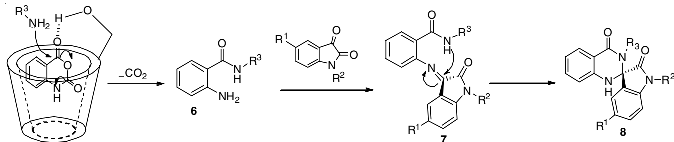
Fig. 1. Plausible mechanistic pathway for reaction for synthesis of spiroindole nucleus
