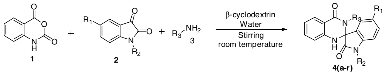
Scheme-I: Synthesis of different spiroindole quinazolines derivatives
