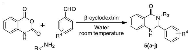
Scheme-II: Synthesis of different dihydro quinazolines derivatives
