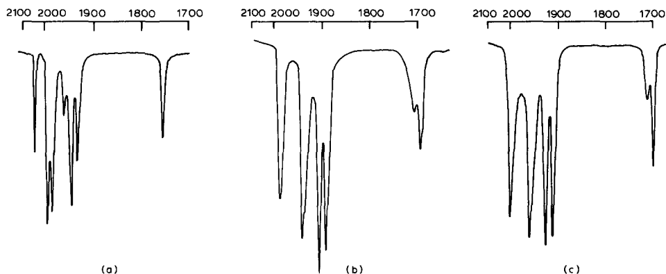
Fig. 1. Cyclohexane solution infrared spectra, in the C–O stretching region, of (a) [\text{Fe}_2(\mu\text{-CO})(\text{CO})_6\{\mu\text{-(MeO)}_2\text{PN(Et)P(OMe)}_2\}] , (b) [\text{Fe}_2(\mu\text{-CO})(\text{CO})_4\{\mu\text{-(MeO)}_2\text{PN(Et)P(OMe)}_2\}_2] , and (c) [\text{Ru}_2(\mu\text{-CO})(\text{CO})_4\{\mu\text{-(MeO)}_2\text{PN(Et)P(OMe)}_2\}_2] .
