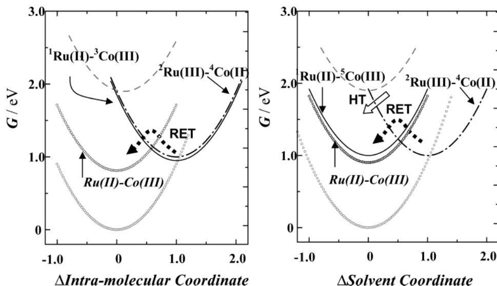
Figure 8. Schematic Gibbs free energy surface of ^3\text{CT}(\text{Ru}) , EET product of [(\text{bpy})_2\text{Ru}^{\text{II}}(\text{tpphz})^4\text{Co}^{\text{II}}(\text{bpy})_2]^{5+} , excitation energy-transfer product of triplet (d-d) state with electronic configurations of 1(\text{d}\pi^6) for \text{Ru}(\text{II}) and 5(\text{d}\pi^4\text{d}\sigma^{*2}) of \text{Co}(\text{III}) , and RET product. The Gibbs free energy surface of the RET product is vertically relaxed to that fully relaxed (gray line). Transitions are shown as in Figure 6.
