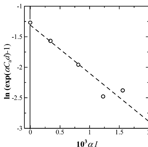
Figure 5. Plot of \ln(\exp(\alpha_2 C_a d) - 1) , against 10^3 \alpha_2 I for a solution of [(bpy)_2Ru^I(tpphz)Co^{III}(bpy)_2]^{5+} .
