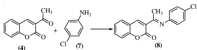
Fig. 3. Synthesis of (E)-3-(1-((4-chlorophenyl)imino)ethyl)-2H-chromen-2-one
