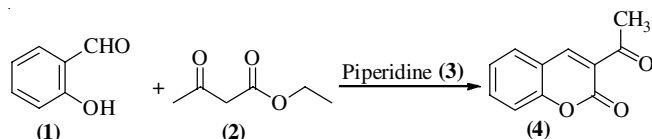
Fig. 1. Synthesis of 3-acetyl-2H-chromen-2-one
