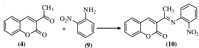
Fig. 4. Synthesis of (E)-3-(1-((2-nitrophenyl)imino)ethyl)-2H-chromen-2-one
