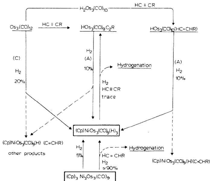
RELATIONSHIPS WITHIN OSMIUM-ALKYNE DERIVATIVES AND COMPLEXES II AND III. OCTANE SOLUTIONS, UNDER HYDROGEN (SEE REF. 19).
