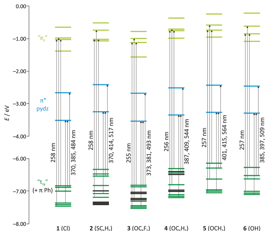
Figure 2. Partial molecular orbital diagram for the complexes [\text{Re}_2(\mu\text{-X})_2(\text{CO})_6(\mu\text{-pydz})] , \text{X} = \text{Cl} (1), \text{SC}_6\text{H}_5 (2), \text{OC}_6\text{F}_5 (3), \text{OC}_6\text{H}_5 (4), \text{OCH}_3 (5), and \text{OH} (6). Orbitals are colored according to their main component: rhenium “ t_{2g} ” orbitals (dark green), pyridazine \pi^* orbitals (light blue), rhenium “ e_g ” orbitals (light green), and phenyl \pi orbitals (black, in complexes 2–4). Arrows correspond to electronic transitions involved in the absorption spectra (computed TD-DFT wavelengths are given). In particular, for each species, values on the left and the right refer to the d–d and the MLCT absorption, respectively.
