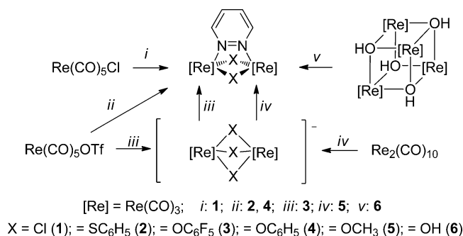
Scheme 1. The Different Synthetic Routes (i–v) Leading to Complexes 1–6
