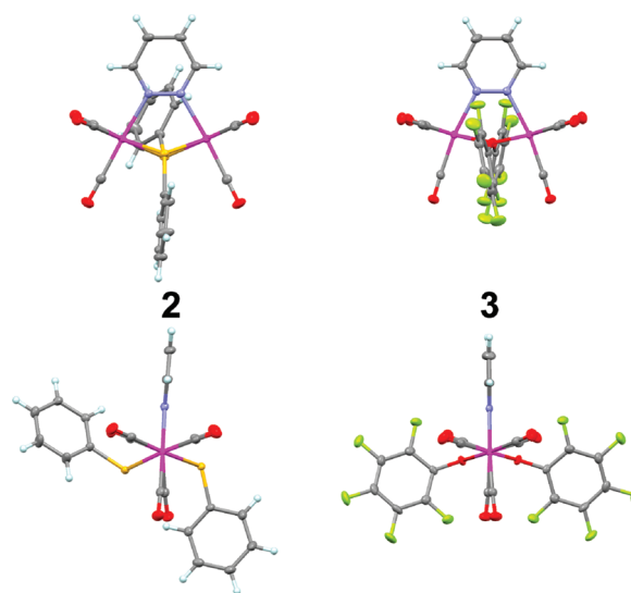
Figure 1. Crystal structures of [\text{Re}_2(\mu\text{-SC}_6\text{H}_5)_2(\text{CO})_6(\mu\text{-pydz})] (2) and [\text{Re}_2(\mu\text{-OC}_6\text{F}_5)_2(\text{CO})_6(\mu\text{-pydz})] (3): frontal and lateral views (upper line and lower line, respectively). Displacement ellipsoids are drawn at the 50% probability level. (Color code: C, gray; H, white; O, red; Re, magenta; and S, yellow.)
