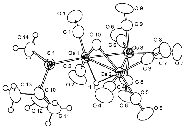
Fig. 5. An ORTEP plot of the molecular structure [\text{Os}_3(\text{CO})_9(\mu\text{-H})(\mu\text{-OH})\{\text{SMe}(\text{Bu}')\}] 11 , showing the atom labelling scheme. Thermal ellipsoids are drawn at the 30% probability level.
