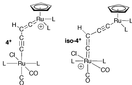
Chart 2. Alternative Alkynyl–Vinylidene Tautomers: 4^+ and iso\text{-}4^+
