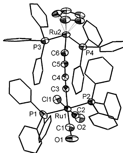
Figure 2. Molecular geometry of 5 in a crystal of 5\cdot 3\text{C}_6\text{H}_6 (phenyl groups simplified, 50% displacement ellipsoids). Selected bond distances (Å) and angles (deg): Ru1–C2 = 1.864(5), Ru1–C1 = 1.927(6), Ru1–C3 = 2.065(4), Ru1–P2 = 2.4071(13), Ru1–P1 = 2.4112(14), Ru1–Cl1 = 2.4564(13), Ru2–C6 = 2.020(5), Ru2–P4 = 2.2824(14), Ru2–P3 = 2.2924(14), C3–C4 = 1.220(6), C4–C5 = 1.370(6), C5–C6 = 1.224(6); C6–Ru2–P4 = 85.16(13), C6–Ru2–P3 = 88.74(14), P4–Ru2–P3 = 102.85(5), C4–C3–Ru1 = 177.1(4), C3–C4–C5 = 178.8(5), C6–C5–C4 = 174.5(5), C5–C6–Ru2 = 176.0(4).
