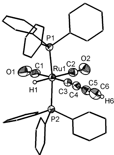
Figure 1. Molecular geometry of 2 in a crystal of 2 \cdot \text{C}_6\text{H}_6 (phenyl groups simplified, 50% displacement ellipsoids). Selected bond distances (Å) and angles (deg): Ru1–C3 = 2.063(3), Ru1–P1 = 2.3557(9), Ru1–P2 = 2.3560(10), C3–C4 = 1.210(4), C5–C6 = 1.176(4), C5–C4 = 1.386(4), Ru1–H1 = 1.57(4), C6–H6 = 0.95(2), P1–Ru1–P2 = 168.00(3), C4–C3–Ru1 = 177.2(3), C6–C5–C4 = 178.7(3), C3–C4–C5 = 178.1(4).
