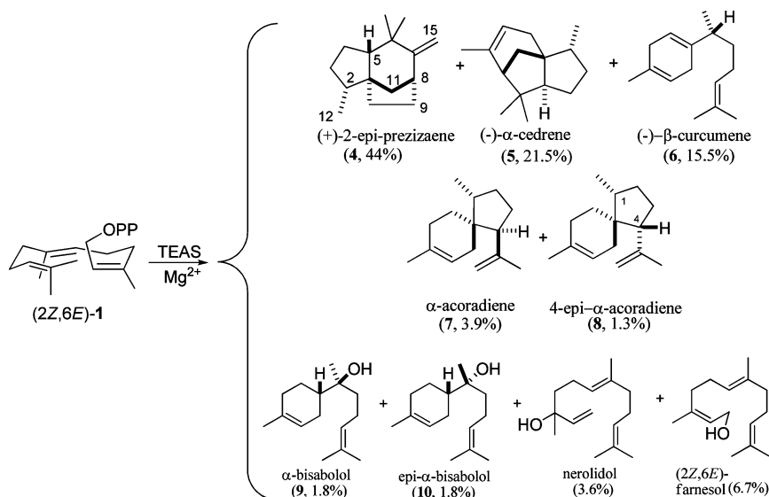
Scheme 1. Sesquiterpenes Produced by Incubations of TEAS with (2 Z ,6 E )-FPP ( 1 ) a
