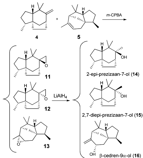
Scheme 2. Chemical Correlation of Cyclization Products 4 and 5 with the Known Compounds 8α,9α-Epoxycedrane ( 13 ), Jinkohol (2-Epi-prezizaan-7β-ol, 14 ), and β-Cedren-9α-ol ( 16 ) by Epoxidation and LiAlH 4 Reduction
