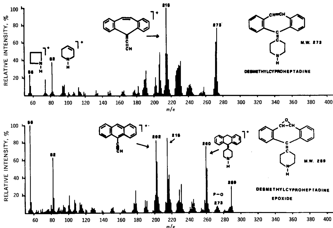
Figure 3—Mass spectrum of IV and VI obtained by introducing the eluted TLC spots by a direct inlet system or by a GLC procedure.
