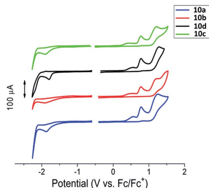
Fig. 1 Cyclic voltammograms for cross-coupling products, 4H-imidazoles 10a–d in a \text{CH}_3\text{CN} solution. Potentials calibrated vs. \text{Fc}/\text{Fc}^+ .
