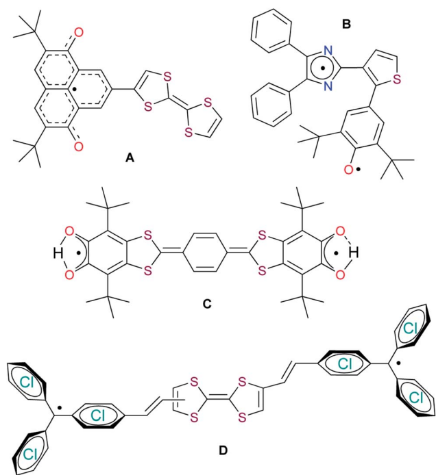
Chart 2 Some electroactive and photoactive dyads and triads based on stable radicals: oxophenalyloxy (A), 10i phenoxyl-imidazolyl (B), 10d,f di- tert -butyl- ortho -semiquinonyl (C), 10e,g and trityl (D). 10b
