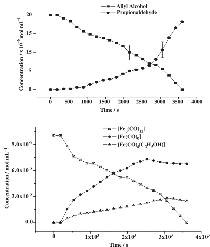
Figure 3. Top: Concentration profiles of propionaldehyde and allyl alcohol during 532 nm photoisomerization of allyl alcohol in hexane with [\text{Fe}_3(\text{CO})_{12}] . Bottom: Concentration profiles of [\text{Fe}_3(\text{CO})_{12}] , [\text{Fe}(\text{CO})_5] , and [\text{Fe}(\text{CO})_4(\text{C}_3\text{H}_5\text{OH})] under the same conditions.
