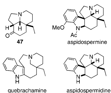
FIGURE 1. Aspidosperma alkaloid targets.
