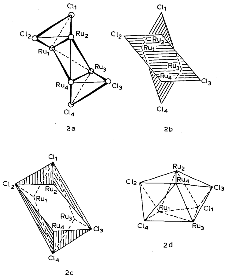
Fig. 2. Idealized view of the framework of [\text{Ru}_4(\mu\text{-Cl})_4(\mu\text{-CO})_2(\text{CO})_8] .
