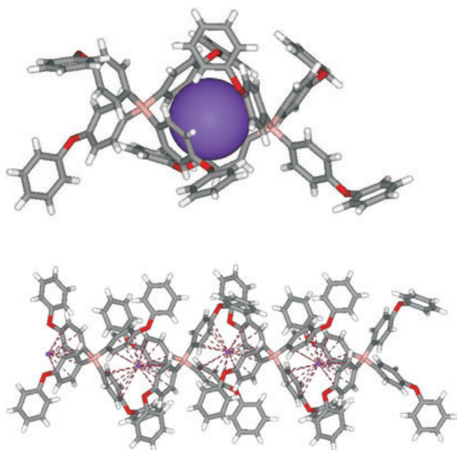
Figure 2. Top: Crystal structure of potassium tetrakis(4-phenoxyphenyl)borate ( \text{K}^+\cdot\mathbf{1} ) showing potassium with VDW radius. Potassium fits perfectly into the cavity formed by the inner aromatic rings of two adjacent borate anions. Bottom: Crystal packing reveals continuous chains of anions connected by strong cation– \pi interactions.
