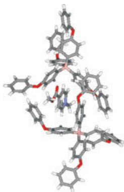
Figure 4. 1-Ethyl-4-(methoxycarbonyl)pyridinium tetrakis(4-phenoxyphenyl)borate complex ( 7-1 ) with offset face-to-face-type \pi\cdots\pi interaction.
