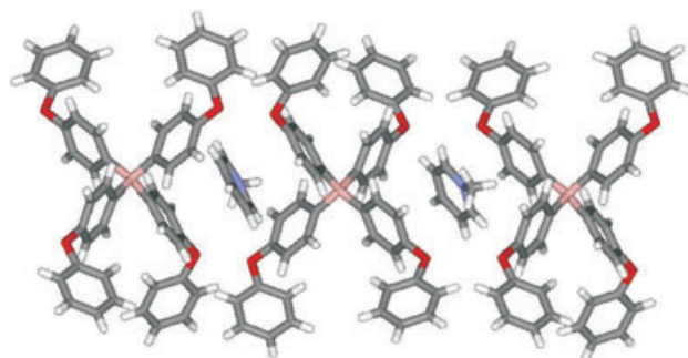
Figure 3. Crystal structure of N -methylpyridinium tetrakis(4-phenoxyphenyl)borate ( \mathbf{6}\cdot\mathbf{1} ). The cation and anion are in face-to-face \pi\cdots\pi contact forming infinite chains.
