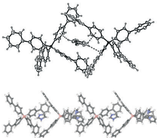
Figure 6. Top: Imidazolium tetrakis(biphenyl)borate complex ( 9-2 ). The complexation involves both offset face-to-face \pi\cdots\pi interactions and edge-to-face C–H \cdots\pi interactions. Bottom: The packing of the anion–cation complexes is similar to that of tetrakis(4-phenoxyphenyl)borate complexes, that is, chainlike.
