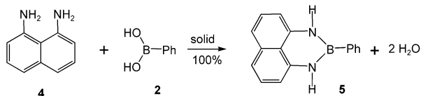
Scheme 2. Quantitative solid-state synthesis of 5 in a ball-mill.
