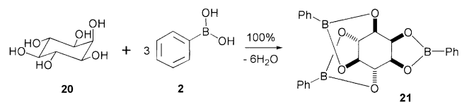
Scheme 9. Quantitative solid-state reaction of myo -inositol with phenylboronic acid.
