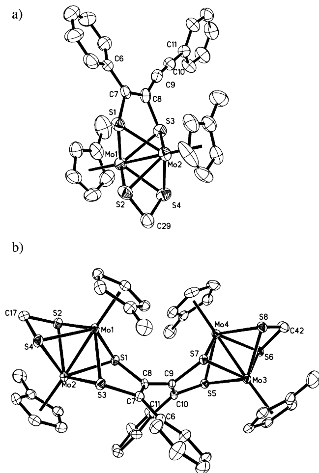
Figure 1. Perspective drawing and numbering scheme for (a) mono-adduct of (MeCpMo \mu -S) 2 S 2 CH 2 and 1,4-diphenylbutadiene ( 5 ) and (b) bis-adduct of (MeCpMo) 2 ( \mu -S) 2 S 2 CH 2 and 1,4-diphenylbutadiene ( 3 ). Thermal ellipsoids are shown at the 50% probability level.
