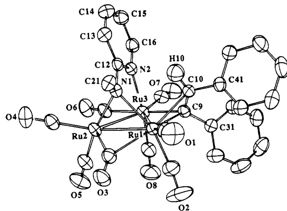
Figure 3. Perspective view of the alkenyl complex \text{Ru}_3(\mu_3\text{-}\eta^2\text{-N-(C}_6\text{H}_5\text{)(C}_5\text{H}_4\text{N))}(\mu\text{-}\eta^2\text{-(C}_6\text{H}_5\text{)CCH(C}_6\text{H}_5\text{))}(\text{CO})_8 ( 4a ). The phenyl ring of the phenylpyridylamido group has been omitted for clarity. Thermal ellipsoids are shown at 30% probability level.
