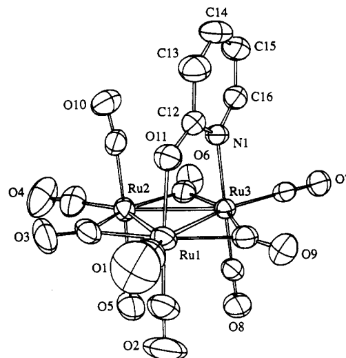
Figure 1. Perspective view of the anion [\text{Ru}_3(\mu\text{-}\eta^2\text{-O-(C}_5\text{H}_4\text{N))}(\text{CO})_{10}]^- (1c). Thermal ellipsoids are shown at 50% probability level.
