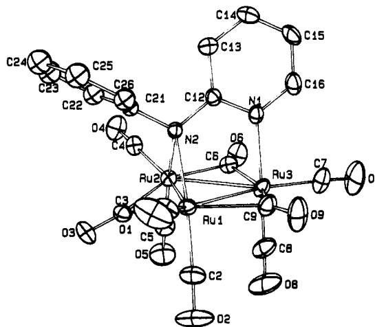
Figure 2. Perspective view of the anion [\text{Ru}_3(\mu_3\text{-}\eta^2\text{-N}(\text{C}_6\text{H}_5)(\text{C}_6\text{H}_4\text{N}))(\text{CO})_9]^- (2a). Thermal ellipsoids are shown at 30% probability level.
