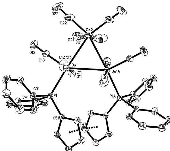
Figure 2. ORTEP diagram of [\text{Os}_3(\text{CO})_{10}(\mu\text{-dppf})] ( 3 ) showing 50% probability thermal ellipsoids. Selected interatomic distances (Å) and angles (deg): \text{Os}(1)\text{--}\text{Os}(2) = 2.8816(3) , \text{Os}(1)\text{--}\text{Os}(1\text{A}) = 2.9507(4) , \text{Os}(1)\text{--}\text{P}(1) = 2.349(1) , \text{Fe}\text{--}\text{C}(\text{av}) = 2.042(1) , \text{P}(1)\cdots\text{P}(1\text{A}) = 5.20 , \text{P}(1)\text{--}\text{Os}(1)\text{--}\text{Os}(2) = 170.27(3) , \text{C}(11)\text{--}\text{Os}(1)\text{--}\text{Os}(2) = 95.3(1) , \text{C}(11)\text{--}\text{Os}(1)\text{--}\text{Os}(1\text{A}) = 80.75(13) , \text{P}(1)\text{--}\text{Os}(1)\text{--}\text{Os}(1\text{A}) = 117.82(3) , \text{C}(13)\text{--}\text{Os}(1)\text{--}\text{Os}(1\text{A}) = 147.0(1) , \text{Os}(1)\text{--}\text{Os}(2)\text{--}\text{Os}(1\text{A}) = 61.594(9) , \text{C}(12)\text{--}\text{Os}(1)\text{--}\text{Os}(2) = 84.08(14) , \text{C}(12)\text{--}\text{Os}(1)\text{--}\text{Os}(1\text{A}) = 92.1(1) , \text{Os}(2)\text{--}\text{Os}(2)\text{--}\text{Os}(1\text{A}) = 59.203(4) .
