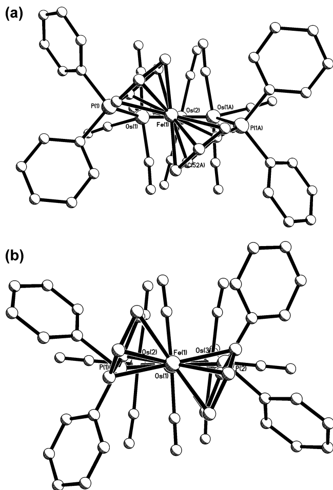
Figure 6. Views of (a) 3 and (b) 2 highlighting the orientation of the ferrocene unit of the dpfp ligand with respect to the triosmium framework.
