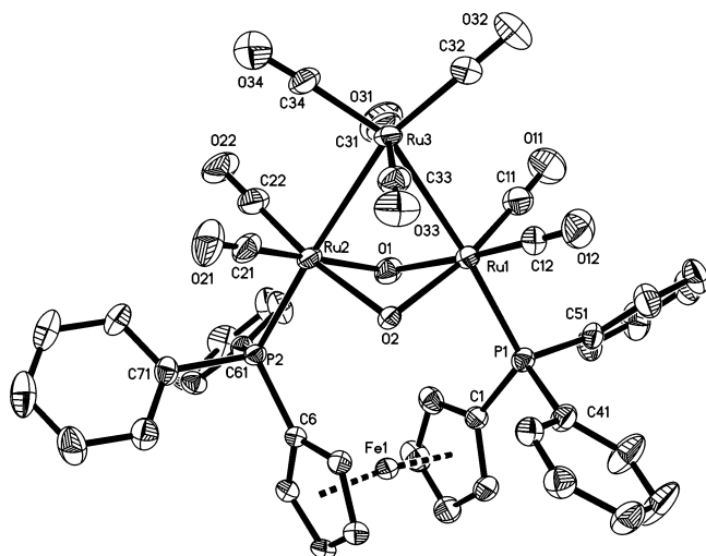
Figure 4. ORTEP diagram of [\text{Ru}_3(\text{CO})_8(\mu\text{-dppf})(\mu\text{-OH})_2] ( 13 ) showing 50% probability thermal ellipsoids. Selected interatomic distances (Å) and angles (deg): \text{Ru}(1)\text{--Ru}(3) = 2.8345(5) , \text{Ru}(1)\text{--Ru}(3) = 2.8317(6) , \text{Ru}(1)\cdots\text{Ru}(2) = 3.0308(6) , \text{Ru}(1)\text{--O}(1) = 2.111(3) , \text{Ru}(2)\text{--O}(1) = 2.119(4) , \text{Ru}(1)\text{--O}(2) = 2.128(3) , \text{Ru}(2)\text{--O}(2) = 2.135(3) , \text{Fe}\text{--C}(\text{av}) = 2.042(6) , \text{Ru}(1)\text{--P}(1) = 2.391(1) , \text{Ru}(2)\text{--P}(2) = 2.365(1) , \text{P}(1)\cdots\text{P}(2) = 5.26 , \text{O}(1)\text{--Ru}(1)\text{--Ru}(3) = 83.7(1) , \text{O}(2)\text{--Ru}(1)\text{--Ru}(3) = 85.85(9) , \text{P}(1)\text{--Ru}(1)\text{--Ru}(3) = 175.16(3) , \text{P}(2)\text{--Ru}(2)\text{--Ru}(3) = 172.41(3) , \text{O}(1)\text{--Ru}(1)\text{--O}(2) = 75.4(1) , \text{O}(1)\text{--Ru}(2)\text{--O}(2) = 75.1(1) , \text{O}(2)\text{--Ru}(2)\text{--Ru}(3) = 85.80(9) , \text{O}(1)\text{--Ru}(2)\text{--Ru}(3) = 83.7(1) , \text{Ru}(2)\text{--Ru}(3)\text{--Ru}(1) = 64.67(1) , \text{Ru}(1)\text{--O}(1)\text{--Ru}(2) = 91.5(1) , \text{Ru}(1)\text{--O}(2)\text{--Ru}(2) = 90.7(1) .
