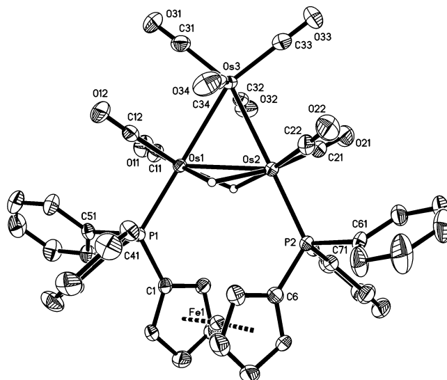
Figure 3. ORTEP diagram of [\text{Os}_3(\text{CO})_8(\mu\text{-dppf})(\mu\text{-H})_2] ( 6 ) showing 50% probability thermal ellipsoids. Selected interatomic distances (Å) and angles (deg): \text{Os}(1)\text{--}\text{Os}(2) = 2.7167(3) , \text{Os}(2)\text{--}\text{Os}(3) = 2.8164(2) , \text{Os}(2)\text{--}\text{Os}(3) = 2.8253(2) , \text{Os}(1)\text{--}\text{P}(1) = 2.3327(9) , \text{Os}(2)\text{--}\text{P}(2) = 2.3511(9) , \text{Fe}\text{--}\text{C}(\text{av}) = 2.0411(4) , \text{P}(1)\text{--}\text{Os}(1)\text{--}\text{Os}(2) = 116.74(2) , \text{P}(2)\text{--}\text{Os}(2)\text{--}\text{Os}(1) = 117.68(3) , \text{P}(1)\text{--}\text{Os}(1)\text{--}\text{Os}(3) = 172.16(2) , \text{P}(2)\text{--}\text{Os}(2)\text{--}\text{Os}(3) = 176.84(3) , \text{C}(11)\text{--}\text{Os}(1)\text{--}\text{Os}(2) = 127.1(1) , \text{C}(12)\text{--}\text{Os}(1)\text{--}\text{Os}(2) = 129.7(1) , \text{C}(21)\text{--}\text{Os}(2)\text{--}\text{Os}(1) = 128.3(1) , \text{C}(22)\text{--}\text{Os}(2)\text{--}\text{Os}(1) = 127.8(1) , \text{Os}(1)\text{--}\text{Os}(2)\text{--}\text{Os}(3) = 61.050(5) , \text{Os}(2)\text{--}\text{Os}(1)\text{--}\text{Os}(3) = 61.378(6) , \text{Os}(1)\text{--}\text{Os}(3)\text{--}\text{Os}(2) = 57.572(6) .
