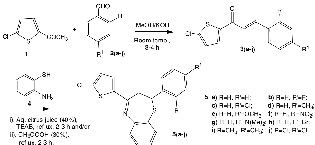
Scheme-I: Schematic diagram for the synthesis of thienyl-benzothiazepines, 5(a-j)
