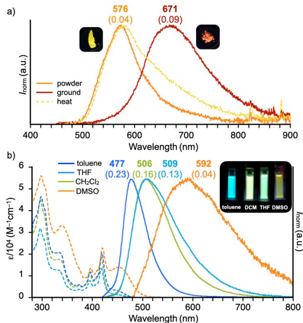
Fig. 4 a) Steady-state PL spectra of powder solids (as prepared), ground, and heated samples; b) Steady-state UV-vis absorption and PL spectra of solutions ( c = 10^{-5} M, \lambda_{ex} = 400 nm) of PSeOZ-DBPHZ-PSeOZ prepared from various solvents. The inset photographs indicate the solutions taken under the irradiation of a UV light ( \lambda = 365 nm).
