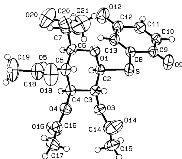
Fig. 3. X-Ray structure of 4 . Arbitrary numbering.
