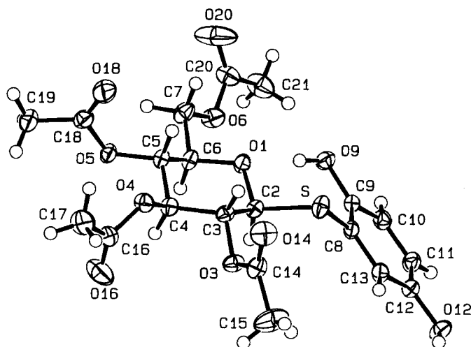
Fig. 1. X-Ray structure of 2 . Arbitrary numbering.
