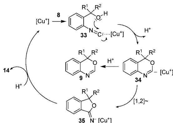
SCHEME 3. Mechanism of the Cu 2 O-Catalyzed Cyclization of Isocyanobenzylalcohols 8
