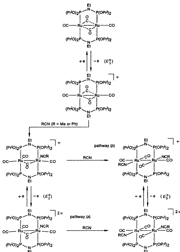
Scheme 1 Possible pathways for the electrochemical oxidation of [\text{Ru}_2(\mu_5b\text{-CO})_2(\text{CO})_2(\mu\text{-etipdp})_2] in organonitrile solvents
