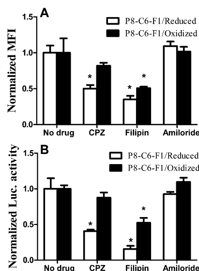
Fig. 9 Effect of endocytosis inhibitors on cellular internalization of Cy5-labelled pDNA (A) and subsequent gene expression (luciferase activity) (B) mediated by the efficient P8-C6-F1 lipopolymer (reduced and oxidized). HeLa cells were pre-treated with chlorpromazine, CPZ (5 \mu\text{g ml}^{-1} ), filipin (1 \mu\text{g ml}^{-1} ) or amiloride (25 \mu\text{g ml}^{-1} ). The observations were statistically significant in comparison with untreated controls (* P < 0.05 , two-tailed Student's t -test).
