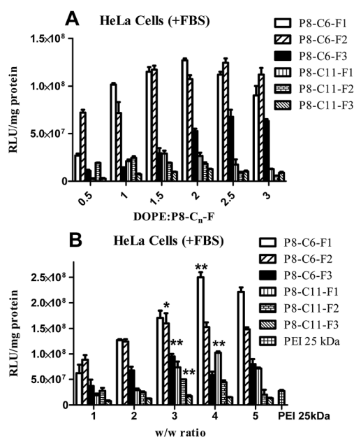
Fig. 3 Optimization of DOPE concentration in lipopolymer formulations while performing transfections at a fixed lipopolymer : DNA ratio (w/w, 2) (A) and maximum luciferase activities obtained from transfection of optimized formulations (B). Transfections were conducted using pGL3-control pDNA (0.4 \mu g) in 10% serum while using BPEI (25 kDa) as a positive control. The luciferase activities were examined for statistical significance in comparison with BPEI (25 kDa) (* P < 0.05 and ** P < 0.01, two-tailed Student's t -test).
