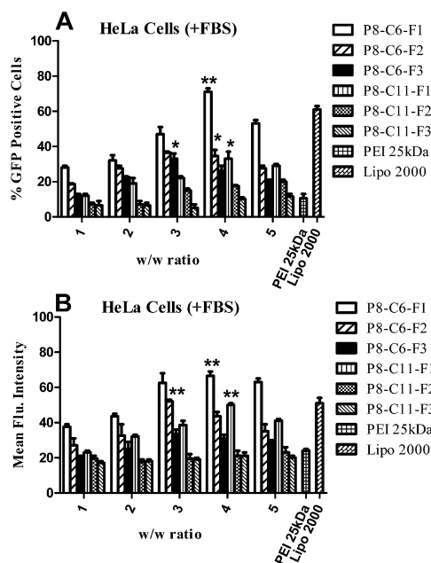
Fig. 4 Flow cytometry analysis of GFP expression for transfections mediated by optimized lipopolymeric formulations as (A) % GFP positive cells and (B) mean intensity of GFP fluorescence (mean flu. intensity). Transfections were performed using pEGFP-C3 pDNA (0.4 \mu g) in 10% serum. The GFP expression was examined for statistical significance in comparison with BPEI (25 kDa) transfections (* P < 0.05 and ** P < 0.01, two-tailed Student's t -test).
