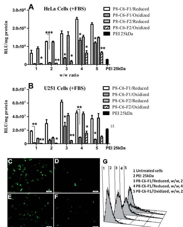
Fig. 6 Comparison of luciferase activities of efficient lipopolymeric formulations (P8-C6-F1 and P8-C6-F2) before and after oxidation of ferrocene in HeLa (A) and U251 cells (B). GFP Expression for transfection with P8-C6-F1 at w/w, 2 in reduced (C and E) and oxidized states (D and F) in HeLa (C and D) and U251 cells (E and F). Flow cytometry histograms of GFP expression in HeLa cells for representative transfections (G). Transfections were performed using pGL3 control/pEGFP-C3 (0.4 \mu g) pDNA in 10% serum. The luciferase activities of oxidized formulations were examined for statistical significance in comparison with those of reduced formulations (* P < 0.05, ** P < 0.01 and *** P < 0.001, two-tailed Student's t -test).
