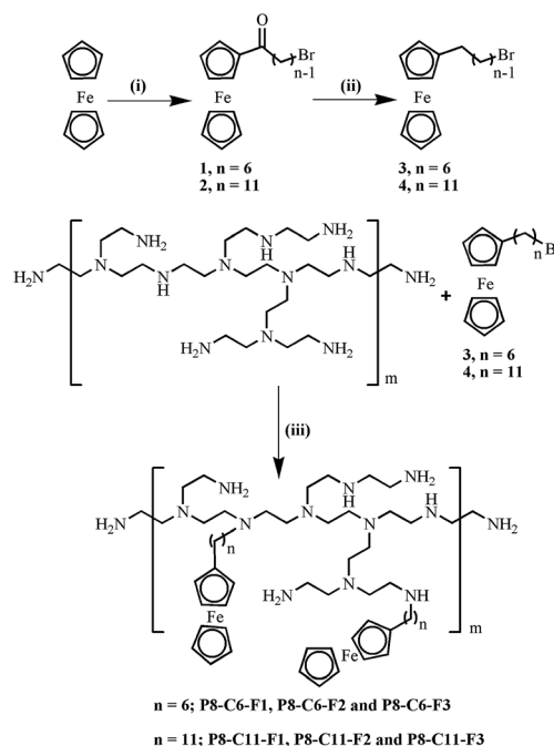
Scheme 1 Synthetic route to the ferrocene modified 0.8 kDa branched poly(ethyleneimine). (i) \omega -Alkanoyl chloride, anhyd. AlCl 3 , CHCl 3 , RT, 12 h; (ii) NaBH 4 /AlCl 3 , THF, RT, 4 h; (iii) MeOH–EtOAc, K 2 CO 3 reflux, 24 h.
