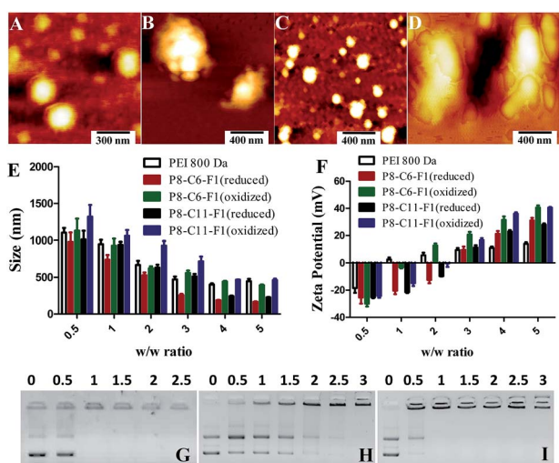
Fig. 2 Representative AFM images of lipopolyplexes (lipopolymer : pDNA, 4 : 1) of P8-C6-F1 (A and B) and P8-C11-F1 (C and D) in reduced (A and C) and oxidized (B and D) states. Particle sizes (E) and Zeta potentials (F) of lipopolyplexes prepared at different lipopolymer : pDNA w/w ratios. Error bars are standard deviations of three independent measurements. Representative gel patterns for pDNA (0.2 \mu g) binding capability of native BPEI (800 Da) (G) P8-C6-F1 co-liposomes before (H) and after (I) oxidation. The numbers above each lane represent lipopolymer : pDNA (w/w) ratios.
