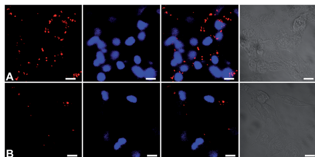
Fig. 8 Representative confocal microscopy images of HeLa cells transfected with P8-C6-F1/Cy5-labelled pDNA (w/w, 2) in the reduced (A) and oxidized (B) states of ferrocene. Panels A and B represent (left to right) pDNA fluorescence, Hoechst 33342 stained nuclei, overlay of the previous two microscopic images and bright field images. Samples were processed after 4 h of lipopolyplex treatment. Scale bar = 10 \mu\text{m} .
