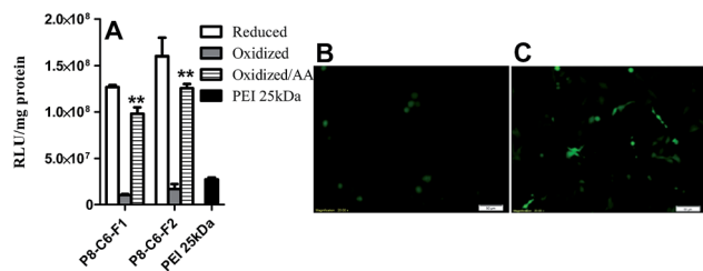
Fig. 7 (A) Luciferase activities of ascorbic acid (AA) treated oxidized lipopolyplexes of P8-C6-F1 (w/w, 2) and P8-C6-F2 (w/w, 3) in HeLa cells in comparison with oxidized (** P < 0.01 ) and reduced lipopolyplexes. GFP expression analysis of HeLa cells transfected with oxidized (B) and AA treated-oxidized P8-C6-F1 (C).
