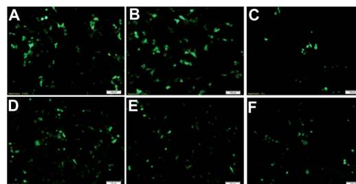
Fig. 5 GFP expression analysis using fluorescence microscopy in HeLa (A–C) and U251 (D–F) cells for the most efficient lipopolymeric formulation, P8–C6–F1 (A and D) in comparison with Lipofectamine 2000 (B and E) and BPEI (25 kDa) (C and F). Transfections were performed using pEGFP-C3 (0.4 \mu g) pDNA at respective optimized w/w ratios for maximum GFP expression. Scale bar = 100 \mu m.
