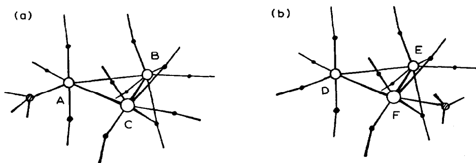
Fig. 5. Molecular structure of [\text{Fe}_3(\text{CO})_{11}\text{PPh}_3] . \text{PPh}_3 substituted on (a) unique Fe atom and (b) on a bridging Fe atom.
