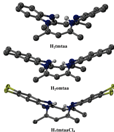
Figure 2. X-ray crystal structures of H 2 tmtaa, H 2 omttaa, and H 2 tmtaaCl 4 , respectively. Thermal ellipsoids are shown at the 50% probability level with hydrogens omitted for clarity with the exception of the amine hydrogens.
