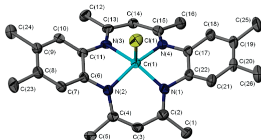
Figure 3. Thermal ellipsoid plot of 2 at 50% probability. Hydrogen atoms omitted for clarity.
