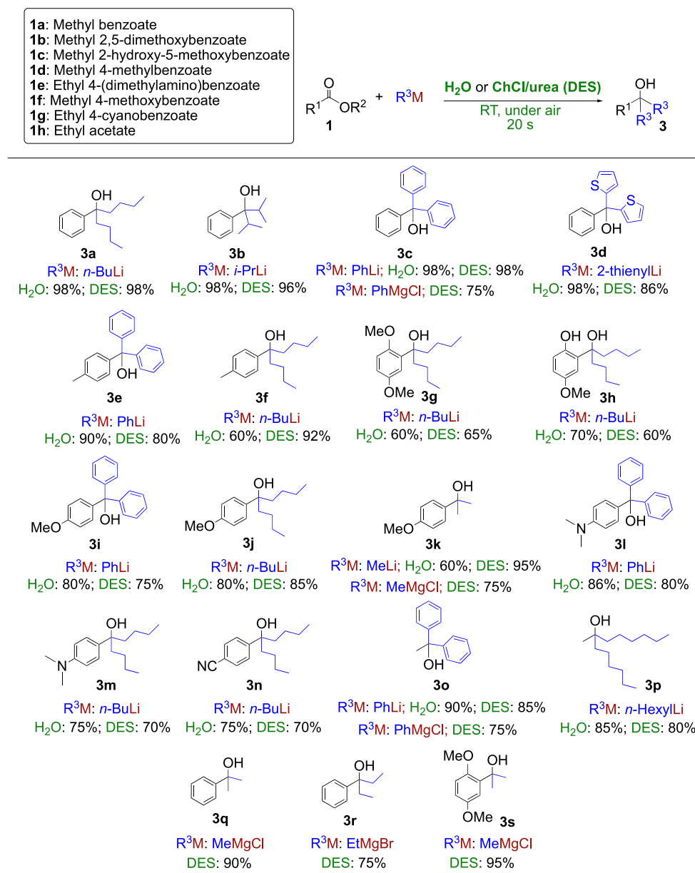
Scheme 2. Synthesis of alcohols 3 by addition of organolithium or Grignard reagents to esters 1 in \text{H}_2\text{O} or in \text{ChCl/urea} , at ambient temperature (RT) under air (reaction conditions: ester: 0.5 mmol; organometallic reagent: 1.25 mmol; \text{H}_2\text{O} : 1 mL; \text{ChCl/urea} : 1 g). The yields reported are for products isolated and purified by column chromatography.
