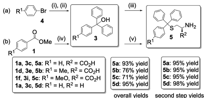
Scheme 3. (a) General route for the synthesis of thioethers; reagents and conditions: (i) n -BuLi, -78^{\circ}\text{C} , 1 h; (ii) \text{Ph}_2\text{CO} , THF, -78^{\circ}\text{C} , 4–6 h, then RT overnight; (iii) cysteamine hydrochloride or L-cysteine, TFA, RT, 3 h. (b) This work: reagents and conditions: (iv) 1 (0.5 mmol), PhLi (1.25 mmol), \text{CHCl}_3/\text{urea} (1 g), RT, under air, 20 s; (v) 3 (0.5 mmol), \text{CHCl}_3/\text{urea} (1 g), TFA (0.2 mL), cysteamine hydrochloride (0.5 mmol) or L-cysteine hydrochloride (0.5 mmol), 2 h.
