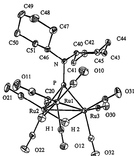
Fig. 1. An ORTEP diagram of \text{H}_2\text{Ru}_3(\text{CO})_9(\mu_3\text{-PNCy}_2) ( 2a ) showing 30% probability thermal ellipsoids. Non-bridging hydrogen atoms or ligands were omitted for clarity. Selected bond lengths (Å) and angles ( ^\circ ): Ru(1)–Ru(2) = 2.9379(3), Ru(1)–Ru(3) = 2.8263(3), Ru(2)–Ru(3) = 2.9664(3), P–N = 1.653(2), Ru(2)–P = 2.3449(7), Ru(1)–P = 2.2833(6), Ru(3)–P = 2.2796(6), C(40)–N–C(46) = 117.41(19).
