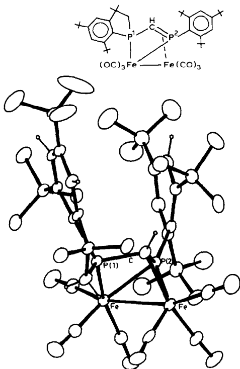
Fig. 1. Molecular structure of [\text{Fe}_2(\text{CO})_6\{\text{ArP}=\text{CHPCH}_2\text{C}(\text{Me}_2)\text{C}_6\text{H}_2^t\text{Bu}_2\}] . Selected bond lengths are: Fe(1)-Fe(2) 2.738(1); P(1)-C 1.771(7); P(2)-C 1.783(6); Fe(1)-P(1) 2.295(2); Fe(2)-P(2) 2.171(2); Fe(1)-P(2) 2.313(2) Å.
