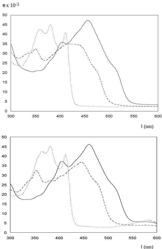
Figure 2. UV-visible spectra of compound 3a (dotted line), 2a (dashed line) and 1a (solid line) in DMSO (upper) and CHCl 3 (lower).
