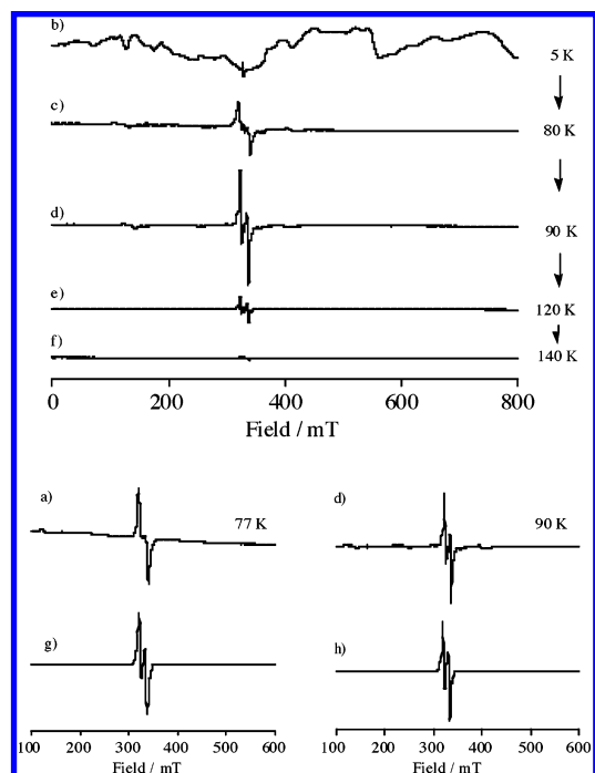
FIGURE 4. (a) ESR spectra obtained by irradiation of bis(diazo) compound 4 – 2\text{N}_2 in 2-methyltetrahydrofuran at 77 K ( \nu_0 = 9.2152 \text{ GHz} ). (b–f) The same spectra observed at 5 (b), 80 (c), 90 (d), 120 (e), and 140 (f) K. (g) Simulated spectra of 4 with S = 1 , g = 2.003 , |D/hc| = 0.0130 \text{ cm}^{-1} , |E/hc| = 0.00 \text{ cm}^{-1} , and \Delta B = 25 \text{ G} . (h) Simulated spectra of 4 with S = 1 , g = 2.003 , |D/hc| = 0.0115 \text{ cm}^{-1} , |E/hc| = 0.00 \text{ cm}^{-1} , and \Delta B = 17 \text{ G} .
