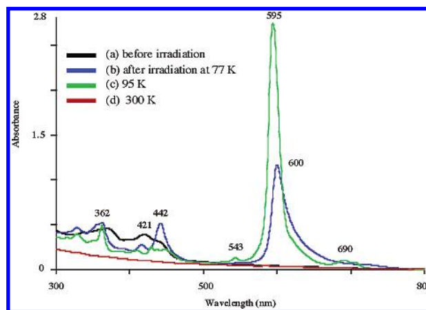
FIGURE 6. UV-vis spectra obtained by irradiation of bis-diazo compound 3-2N 2 . (a) Spectra of 3-2N 2 in 2-methyltetrahydrofuran at 77 K. (b) Sample from part a after irradiation ( \lambda > 350 nm). (c–d) Sample from parts a,b after thawing to 95 (c) and 300 (d) K.
