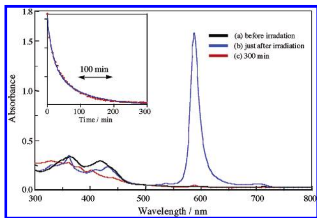
FIGURE 9. Absorption of transient products formed during irradiation of bis(diazo) compound 3 –2N 2 in degassed benzene at room temperature, recorded (a) before irradiation, (b) immediately after irradiation, and (c) 300 min after excitation. Inset shows the time course of the absorption at 588 nm.
