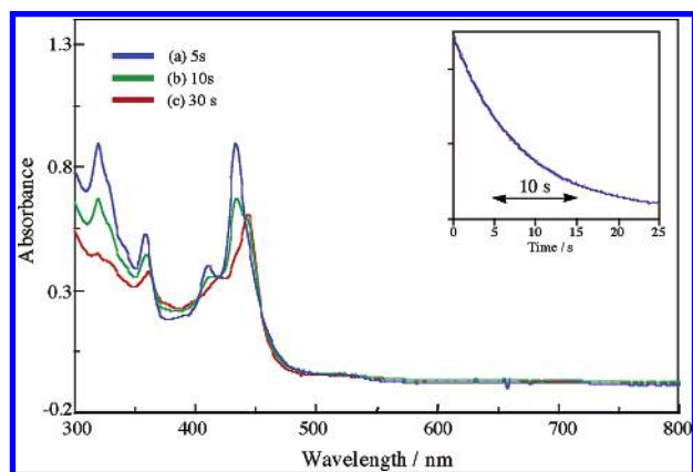
FIGURE 8. Absorption of transient products formed during irradiation of monodiazocompound 2 -N 2 in degassed benzene at room temperature, recorded (a) 5, (b) 10, and (c) 30 s after excitation. Inset shows the time course of the absorption at 433 nm (oscilloscope trace).
