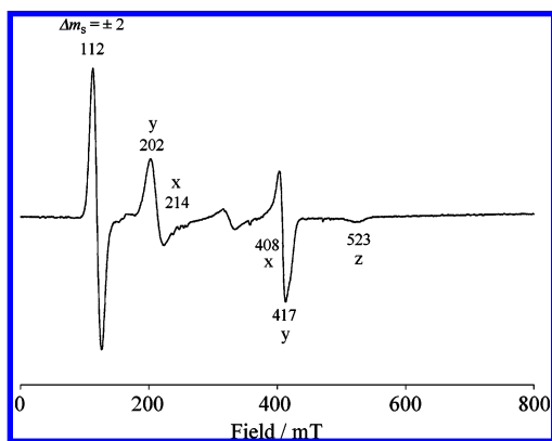
FIGURE 1. ESR spectra obtained by irradiation of monodiazomethane 2-N_2 in 2-methyltetrahydrofuran at 77 K. The microwave frequency ( \nu_0 ) was 9.1327 GHz.
