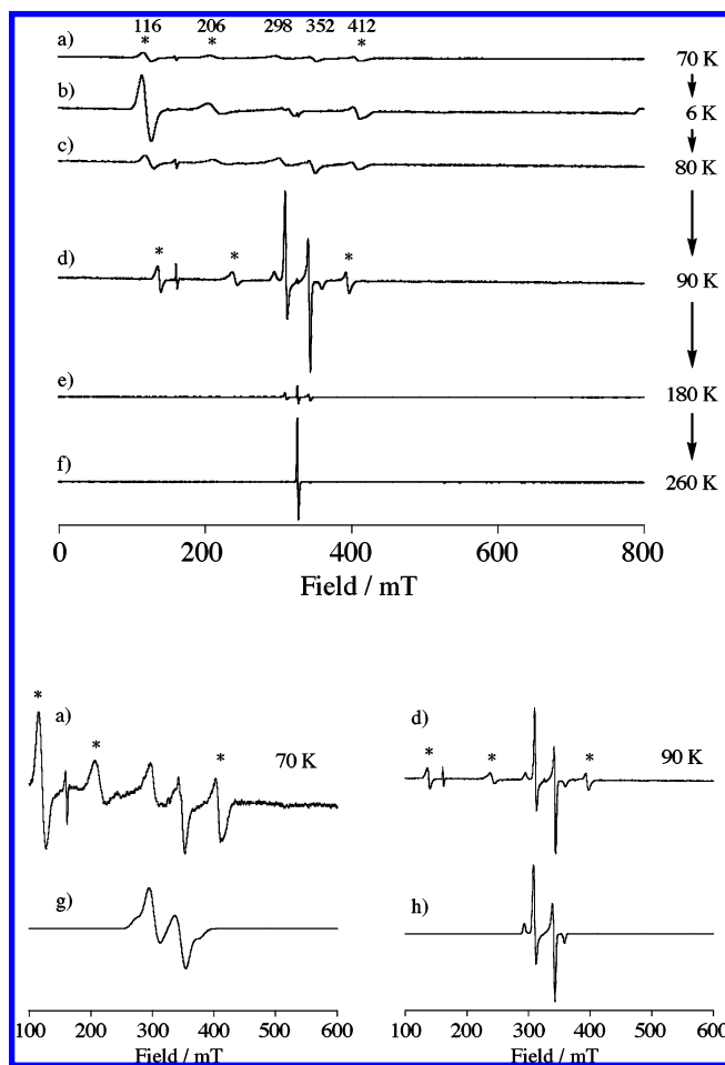
FIGURE 2. (a) ESR spectra obtained by irradiation of bis(diazo) compound 3-2N_2 in 2-methyltetrahydrofuran at 70 K ( \nu_0 = 9.1320 \text{ GHz} ). (b–f) The same spectra observed at 6 (b), 80 (c), 90 (d), 180 (e), and 260 (f) K. (g) Simulated spectra of ^3\mathbf{3} with S = 1 , g = 2.003 , |D/hc| = 0.0474 \text{ cm}^{-1} , |E/hc| = 0 \text{ cm}^{-1} , and line width ( \Delta B ) of 68 G. (h) Simulated spectra of ^3\mathbf{3} with S = 1 , g = 2.003 , |D/hc| = 0.0306 \text{ cm}^{-1} , |E/hc| = 0.00 \text{ cm}^{-1} , and \Delta B = 18 \text{ G} . Signals marked with asterisks (*) are due to a monocarbene.
