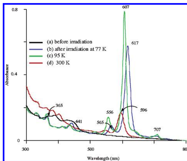
FIGURE 7. UV-vis spectra obtained by irradiation of bis-diazo compound 4-2N 2 . (a) Spectra of 4-2N 2 in 2-methyltetrahydrofuran at 77 K. (b) Sample from part a after irradiation ( \lambda > 350 nm). (c–d) Sample from parts a,b after thawing to 95 (c) and 300 (d) K.
