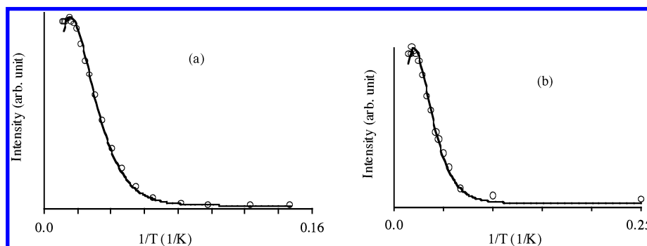
FIGURE 3. Plots of the intensities of the ESR signals (a) at 298 mT due to thermally populated 3 vs reciprocal of temperature (6–75 K), and (b) at 340 mT due to thermally populated 4 vs reciprocal of temperature (4.3–70 K).
