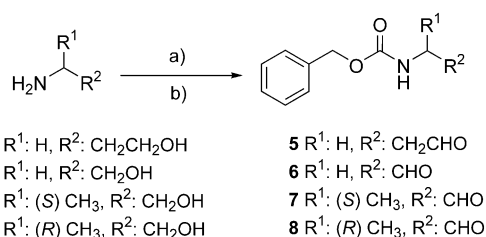
Scheme 1. Synthesis of acceptor aldehydes 5–8 : a) Cbz-OSu dioxane/H 2 O 4/1; b) Swern or IBX oxidation.
