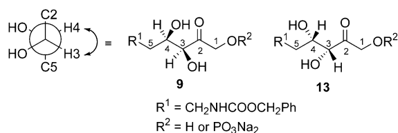
Scheme 3. Main conformer of compounds 9 and 13 .
