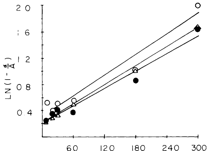
Figure 8—Linear plot of -\ln(1 - \alpha/A) against reaction time at various temperatures. Key: ( \bullet ) 85°C; ( \Delta ) 90°C; ( \circ ) 95°C.
