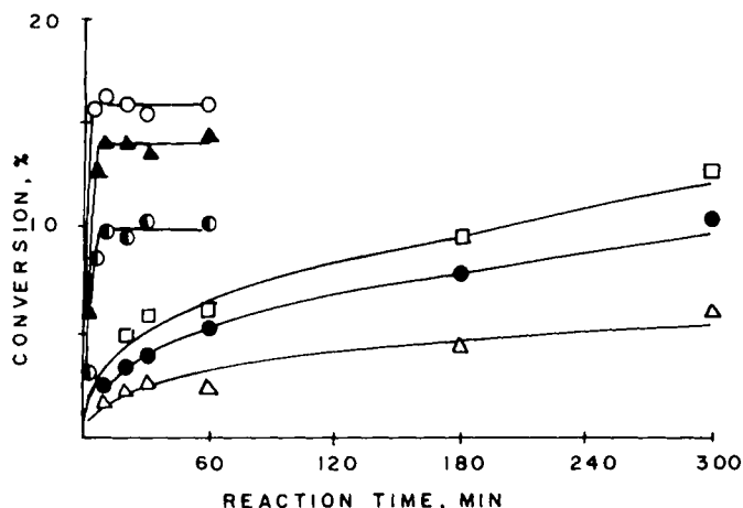
Figure 7—Influence of temperature on the reaction kinetics of equimolar sulfacetamide and phthalic anhydride compacts prepared at 3581 kg/cm 2 . Key: ( \Delta ) 85°C; ( \bullet ) 90°C; ( \square ) 95°C; ( \bullet ) 100°C; ( \blacktriangle ) 105°C; ( \circ ) 110°C.
