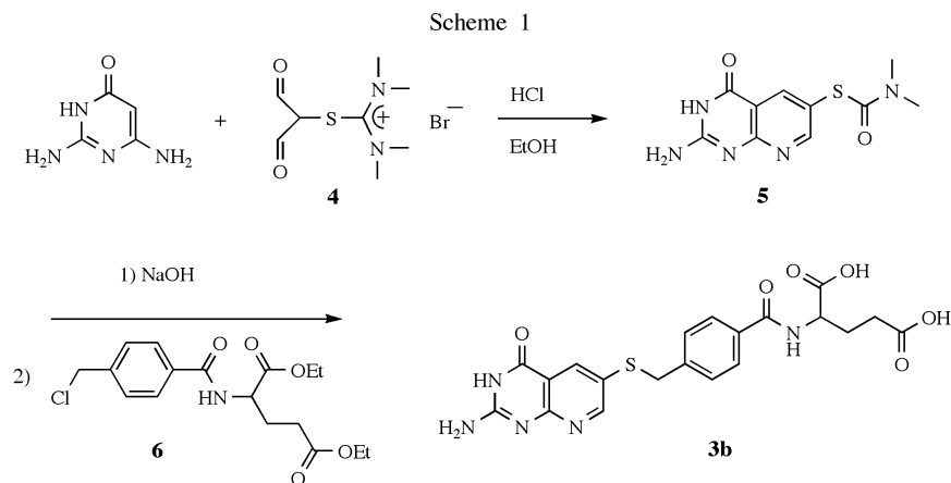
Synthetic Route to 9-Thia-5,10-dideazafolic Acid.
