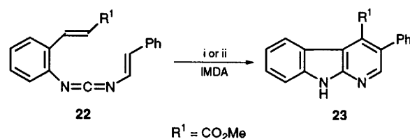
Scheme 3 Reagents and conditions: i, (A) ZnCl 2 , CH 2 Cl 2 , room temp.; ii, (B), 140 °C in xylene
