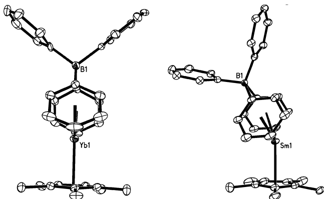
Figure 2. Side-on view of (\text{C}_5\text{Me}_5)\text{Yb}(\mu\text{-}\eta^6\text{:}\eta^1\text{-Ph})_2\text{BPh}_2 , 3 , and (\text{C}_5\text{Me}_5)\text{Sm}(\mu\text{-}\eta^6\text{:}\eta^1\text{-Ph})_2\text{BPh}_2 , 4 . Hydrogen atoms have been excluded for clarity.
