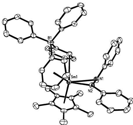
Figure 5. Thermal ellipsoid plot of (\text{C}_5\text{Me}_5)(\text{BPh}_4)\text{Sm}(\text{N}_2\text{Ph}_2) , 9 , with the probability ellipsoids drawn at the 50% level. Hydrogen atoms have been excluded for clarity.
