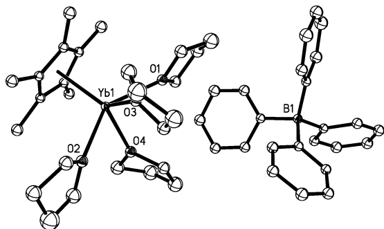
Figure 3. Thermal ellipsoid plot of [(\text{C}_5\text{Me}_5)\text{Yb}(\text{THF})_4][\text{BPh}_4] , 5 , with the probability ellipsoids drawn at the 50% level. Hydrogen atoms have been excluded for clarity.
