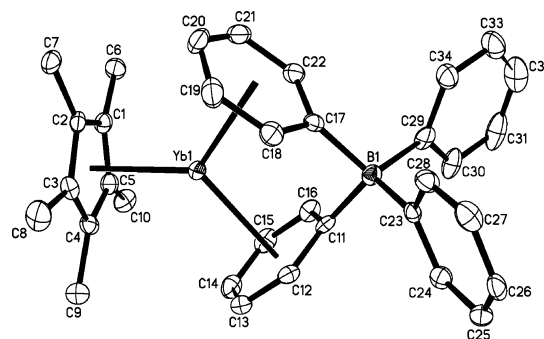
Figure 1. Thermal ellipsoid plot of (C 5 Me 5 )Yb( \mu - \eta^6 : \eta^1 -Ph) 2 BPh 2 , 3 , with the probability ellipsoids drawn at the 50% level. Hydrogen atoms have been excluded for clarity. (C 5 Me 5 )Sm( \mu - \eta^6 : \eta^1 -Ph) 2 BPh 2 , 4 , is numbered similarly.
