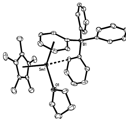
Figure 4. Thermal ellipsoid plot of (\text{C}_5\text{Me}_5)\text{Sm}[(\mu\text{-}\eta^6\text{:}\eta^1\text{-Ph})(\mu\text{-}\eta^1\text{:}\eta^1\text{-Ph})\text{BPh}_2](\text{THF}) , 6 , with the probability ellipsoids drawn at the 50% level. Hydrogen atoms have been excluded for clarity.
