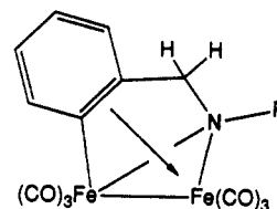
7a: R = i -Pr
