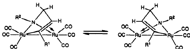
Figure 6. Fluxional behavior of 3 in solution.
