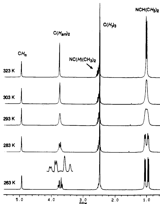
Figure 4. Temperature-dependent ^1\text{H} NMR spectra of 3a in \text{CDCl}_3 at 250.1 MHz.
