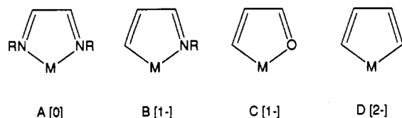
Figure 1. (Hetero)metallacyclopentadiene systems. The formal charge of the ligands is given between brackets.
