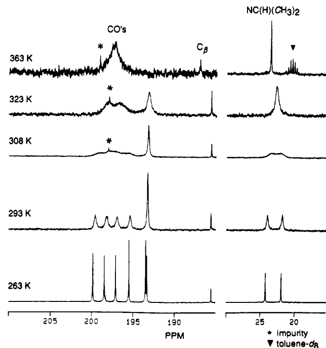
Figure 5. Temperature-dependent ^{13}\text{C} NMR spectra of 3a in \text{CDCl}_3 (263–323 K) or toluene- d_8 (363 K) at 62.9 MHz.
