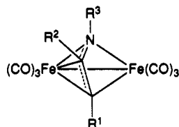
8a: \text{R}^1 = \text{C}(\text{O})\text{OCH}_3 ; \text{R}^2 = \text{C}(\text{O})\text{OCH}_3 ; \text{R}^3 = \text{C}(\text{C}_6\text{H}_5)=\text{C}(\text{CH}_3)_2 8b: \text{R}^1 = \text{H} ; \text{R}^2 = \text{H} ; \text{R}^3 = t\text{-Bu}
